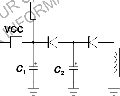
Figure 61. Split V_{CC} Supply
