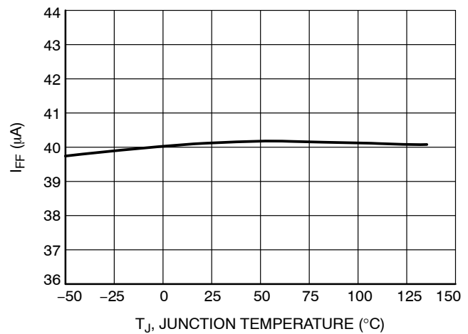
Figure 37. Line Feedforward Current on CS Pin (@ V DS = 2 V) vs. Temperature
